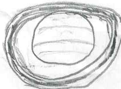
Saturn
